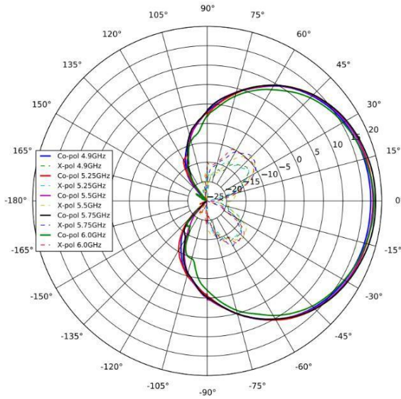
5 GHz Azimuth
