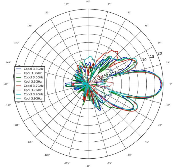
3 GHz Elevation
