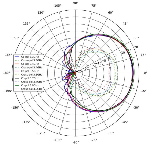
3 GHz Azimuth
