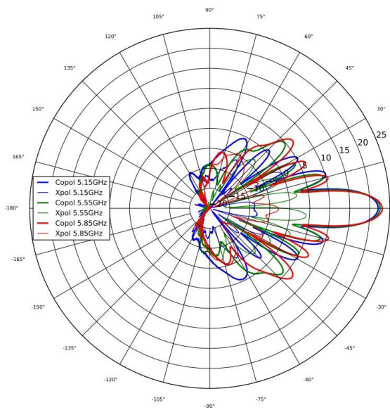
5 GHz Azimuth
