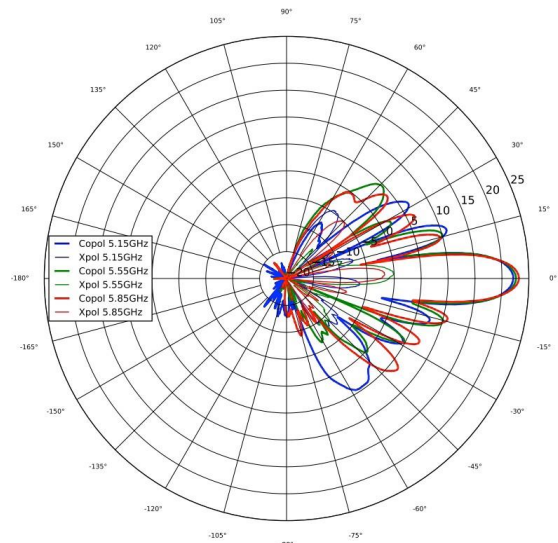
5 GHz Elevation
