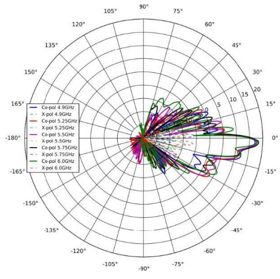
5 GHz Elevation
