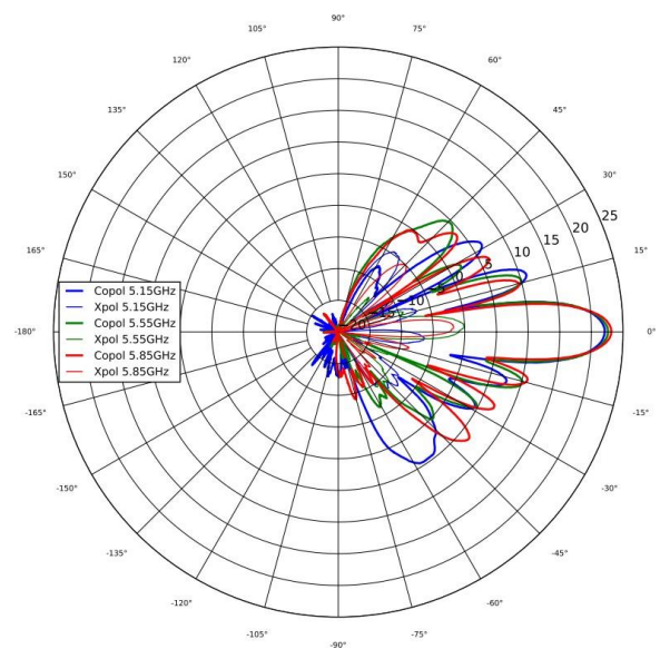
5 GHz Elevation
