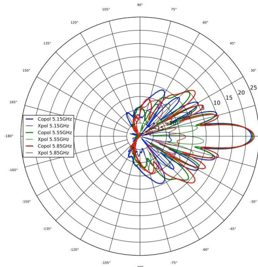
5 GHz Azimuth
